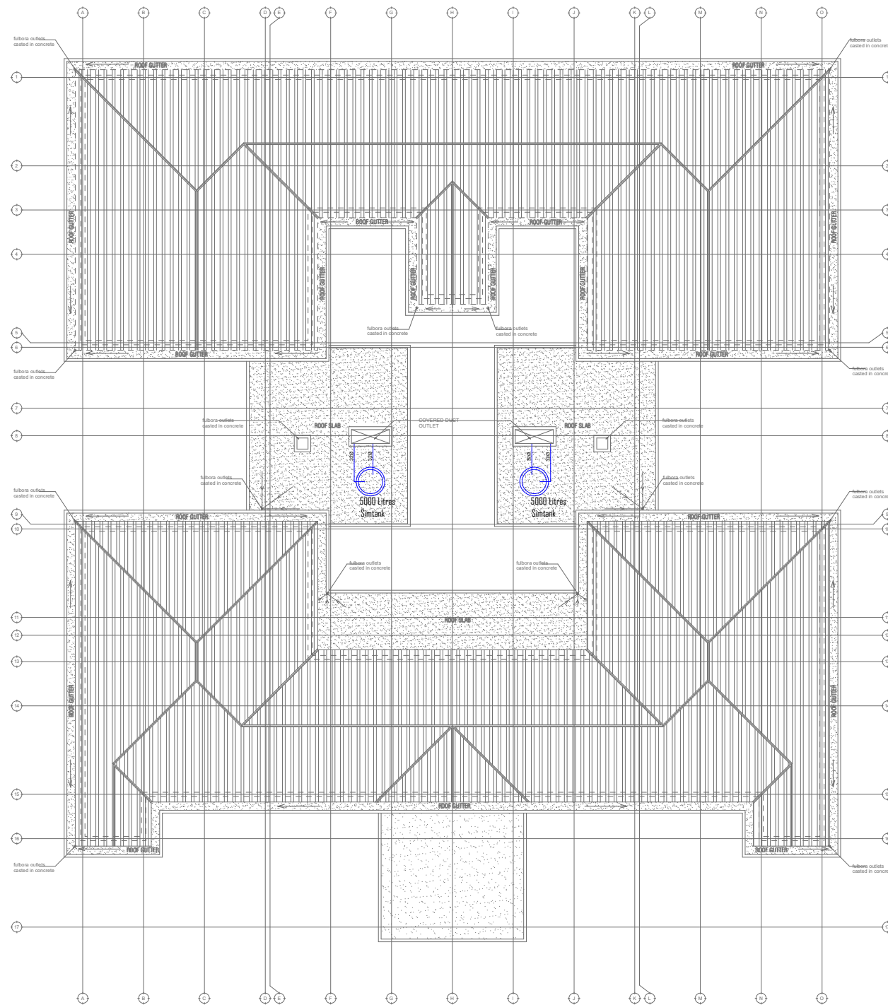
ROOF PLAN
